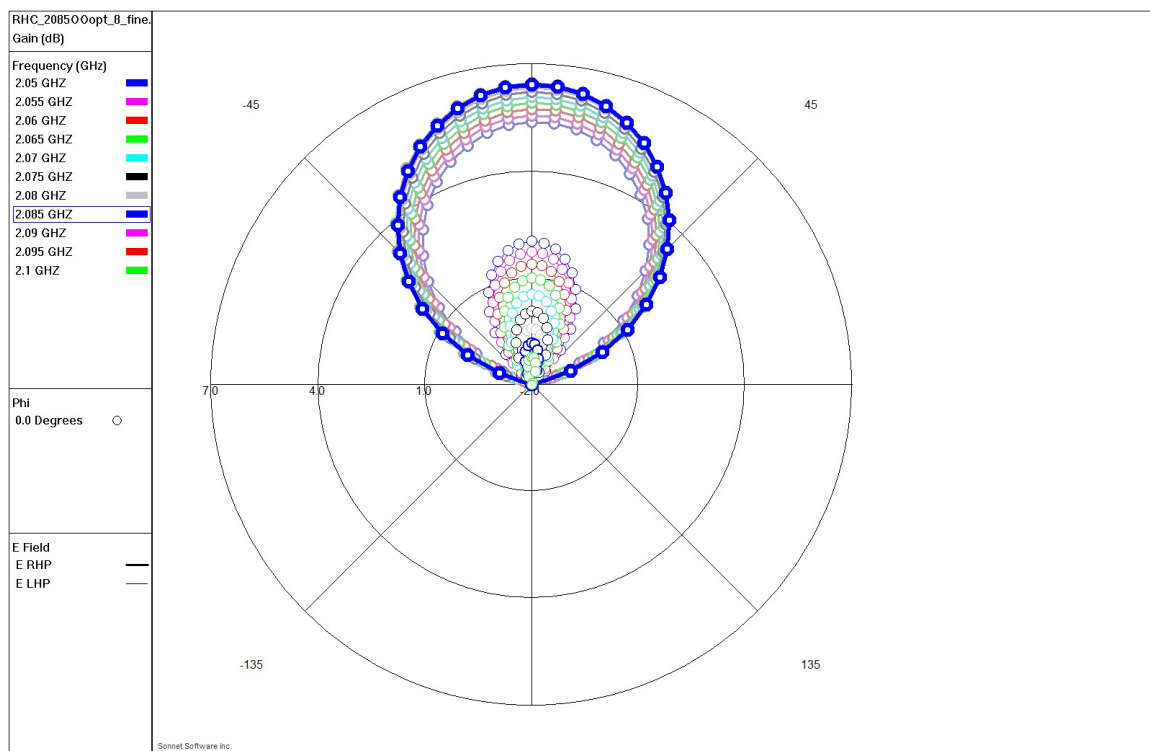
Figure 4: Simulation results of antenna pattern 0°, RHC (bold) vs. LHC
