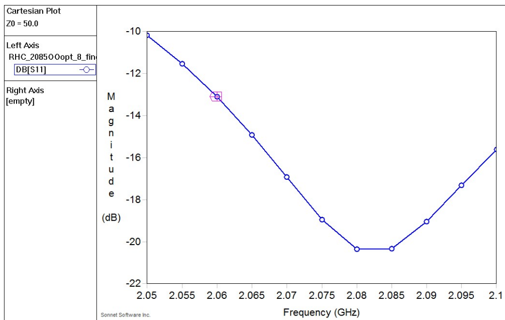
Figure 3: Simulation results of impedance matching (S11, blue)
