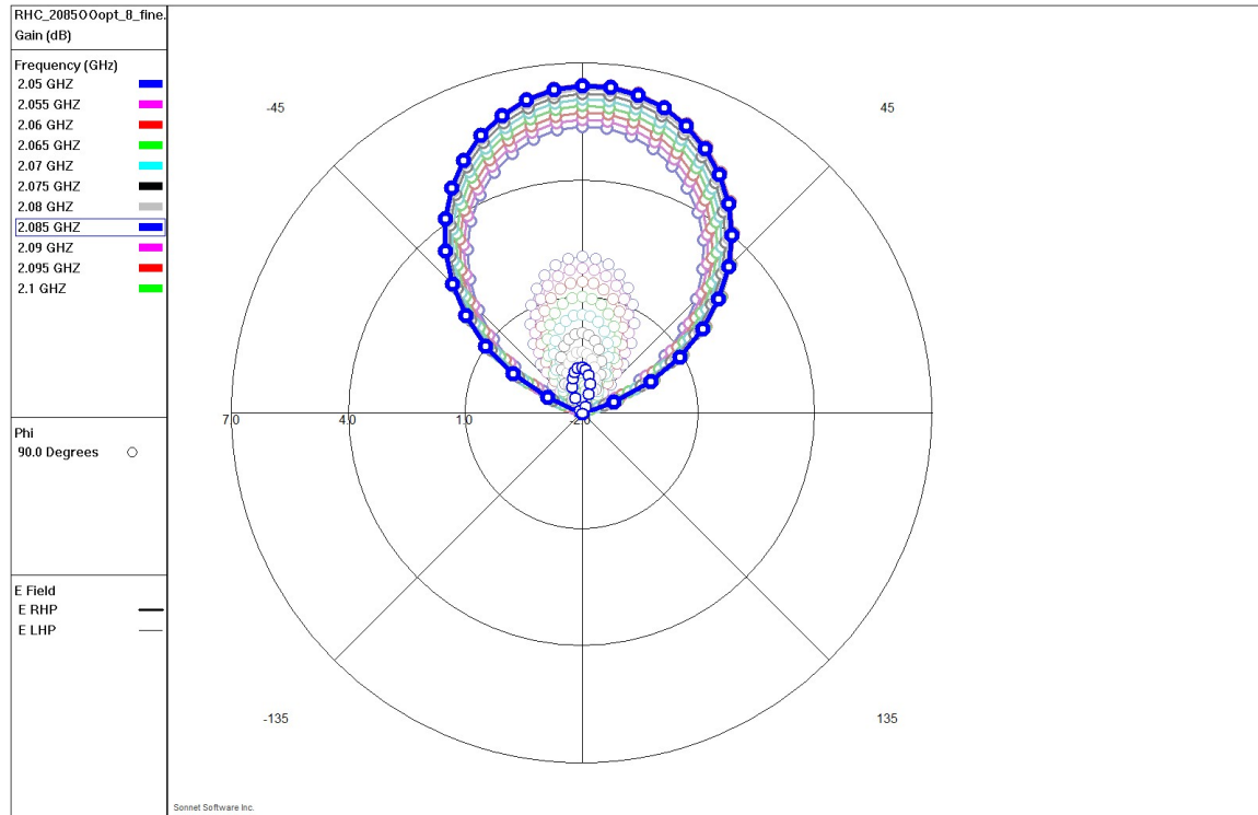
Figure 5: Simulation results of antenna pattern, 90° RHC (bold) vs. LHC
